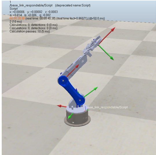
Fig. 11. Forward Position Simulation
